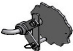
Locking pin in cleating rod (for non-insulated doors only)
